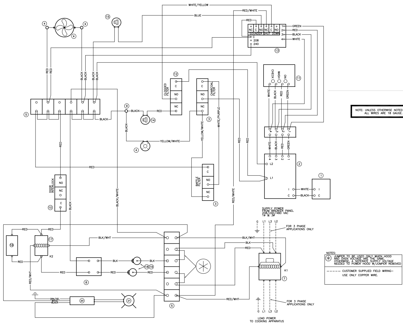
WIRING DIAGRAM PO-VH W-INTRLKS/UV/ILS 208-240/60/1 MANUAL RESTART INSTALLATION ONLY
