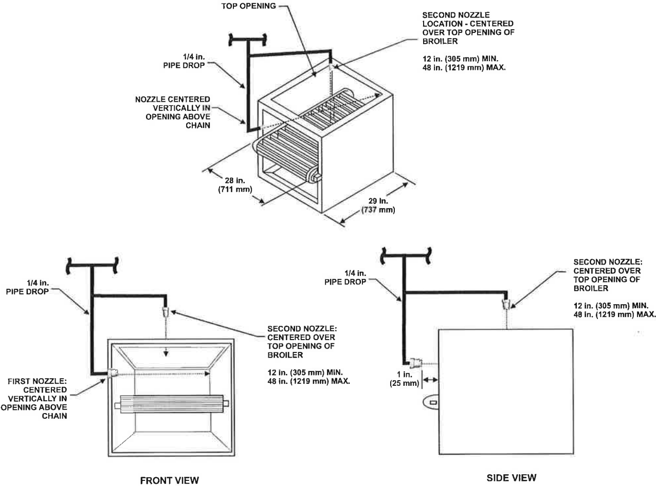
Figure 3-21. ADP Nozzle Installation for Open-Top Chain Broiler
