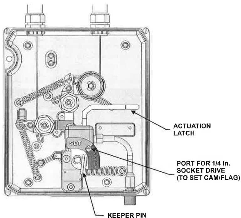
Figure 4-85. Latch Shown in "Set" Position
