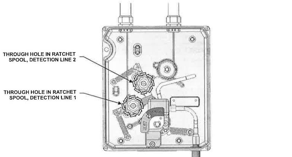
DETECTION BEAMS IN RELEASED POSITION
