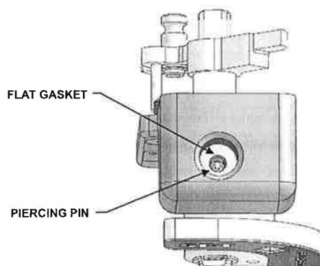
Figure 4-92. Valve Body with Flat Gasket
