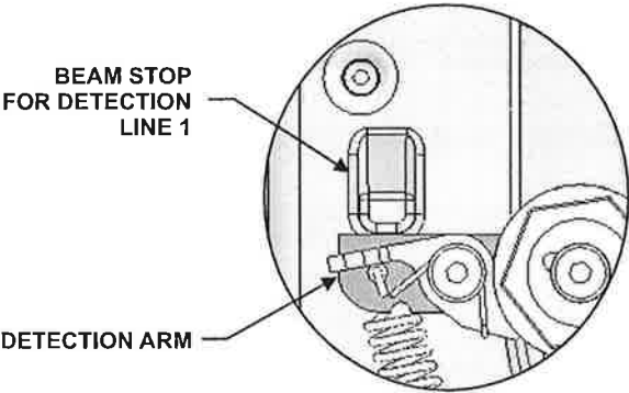
Figure 5-7. Detection Beam Stops
