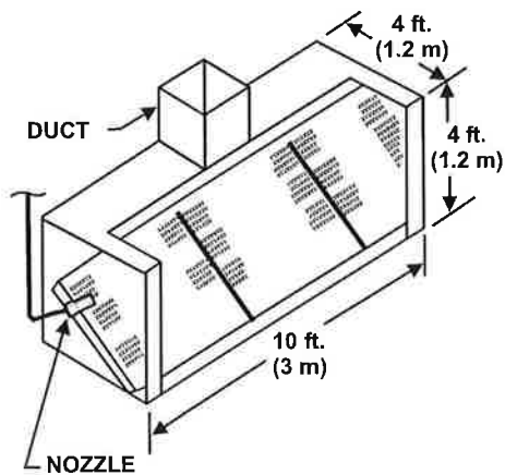
SINGLE FILTER BANK COVERAGE 10 ft. (3 m) PLENUM
