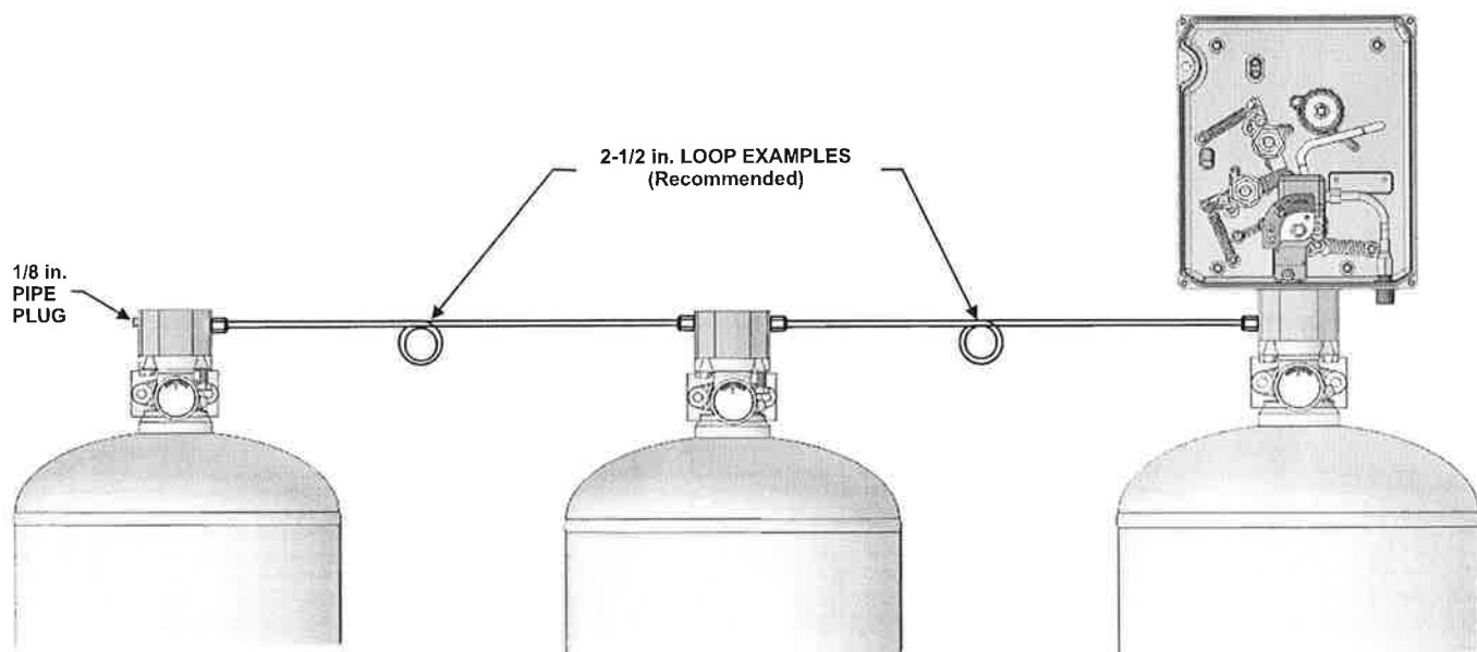
Figure 4-16. Example of Copper Tubing Loop Method
