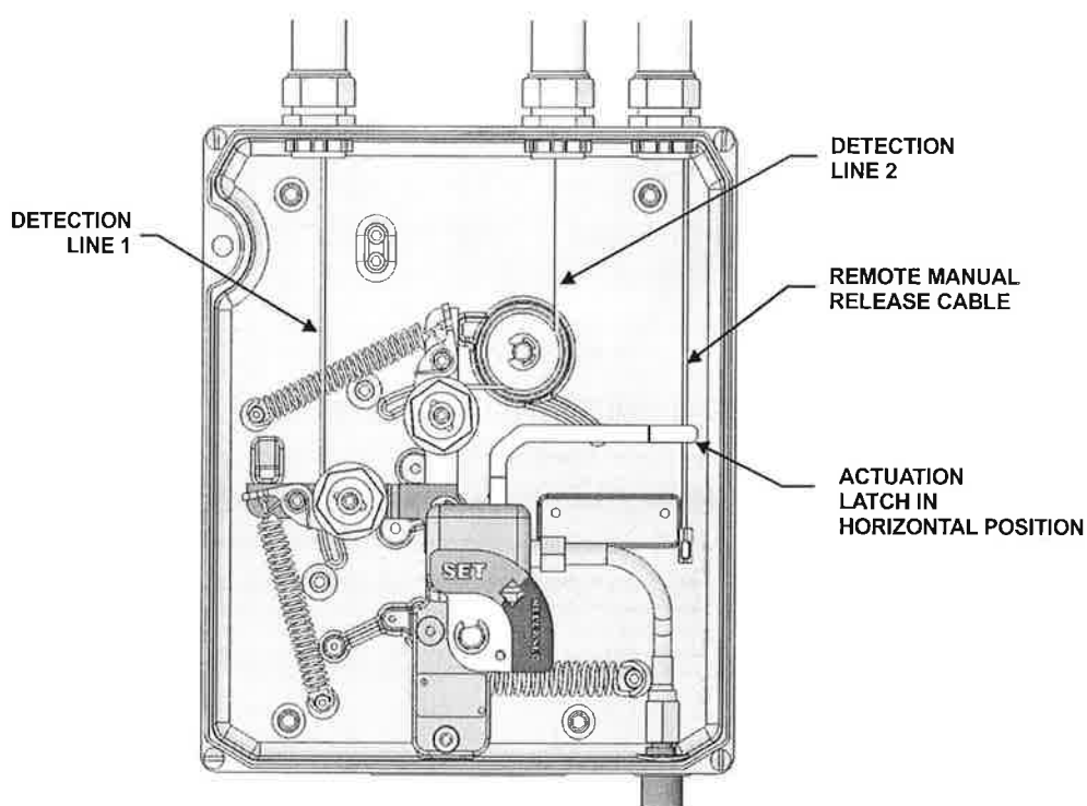
Figure 4-84. Position of Detection Beams in 'Set' Position
