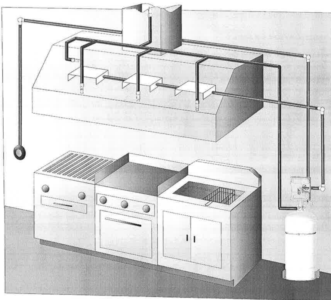
Figure 1-1. Typical Range Guard Wet Chemical System
