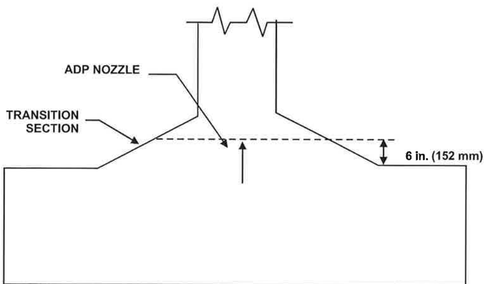
Figure 3-36. Transitional Duct
