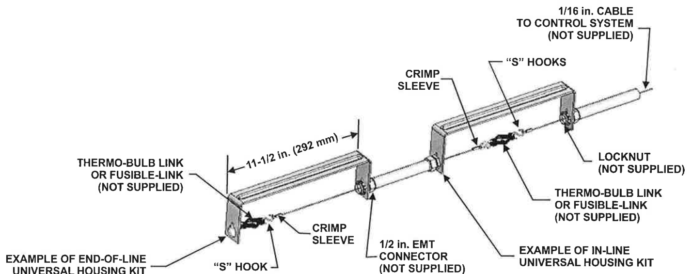
Figure 2-28. Example of End-of-line and In-line Universal Link Housing Kit, P/N 120064
