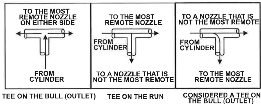
Figure 3-38. Tees
