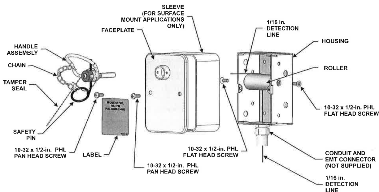
Figure 4-56. Remote Manual Release Pull Station, Pull-to-Trip (EMT/Conduit at Bottom)
