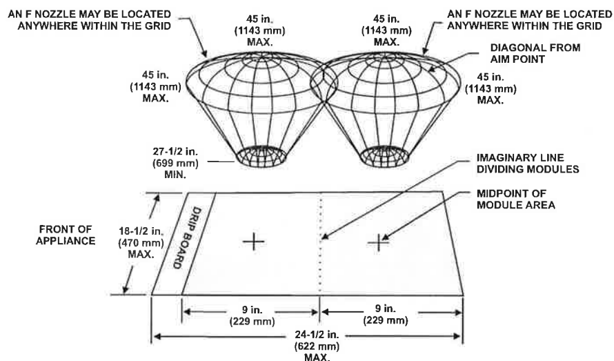
SIDE VIEW
