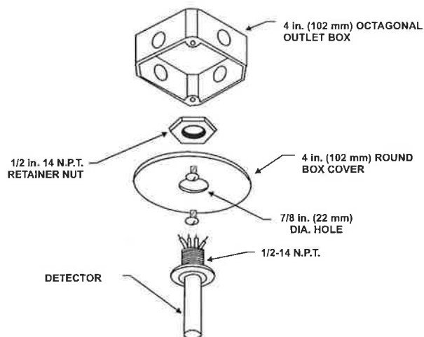
SERIES 27120 AND 27121 DETECT-A-FIRE
