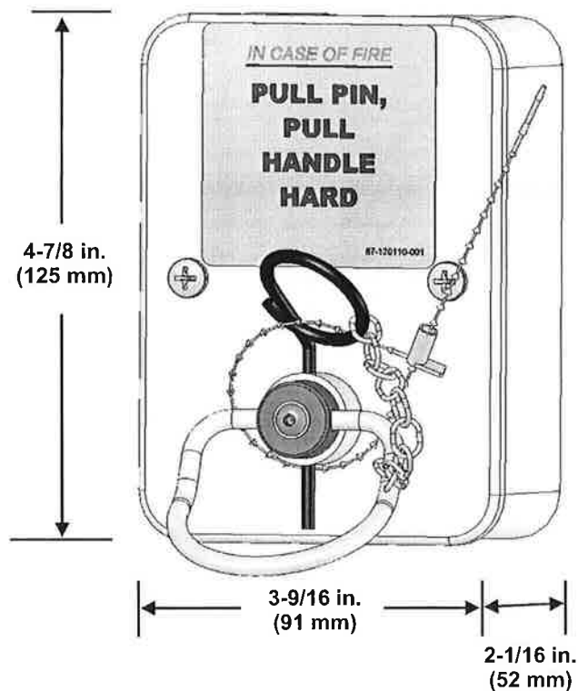
Figure 2-35. Remote Manual Release Pull Station, P/N 87-120110-001
