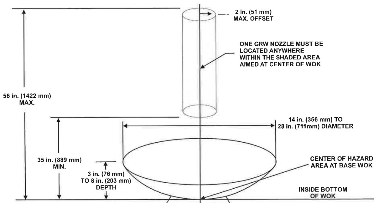
Figure 3-23. Wok
