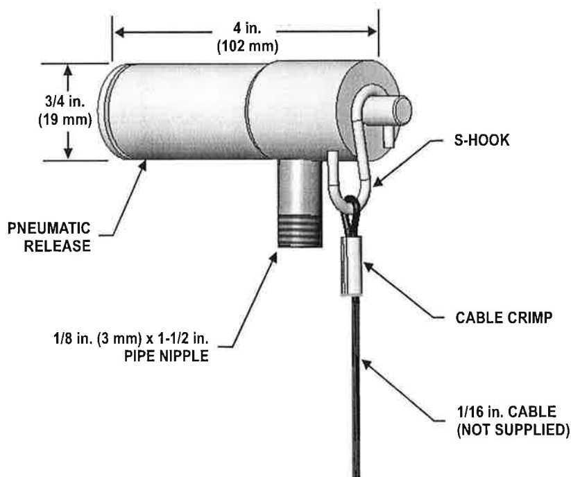
Figure 2-39. Pressure Operated Release, P/N 9189412
